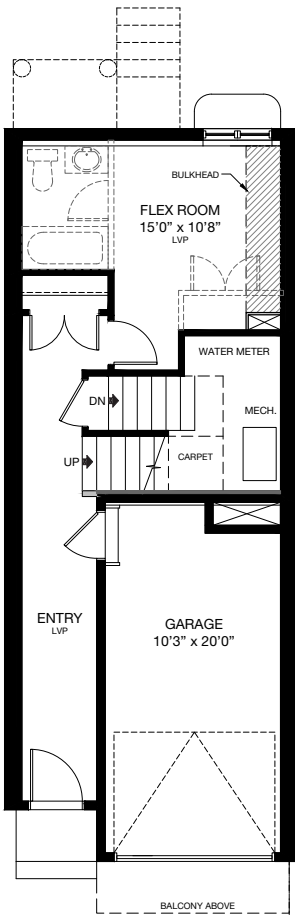
ENTRY LEVEL WATER METER Area: 372 Sq.Ft.
