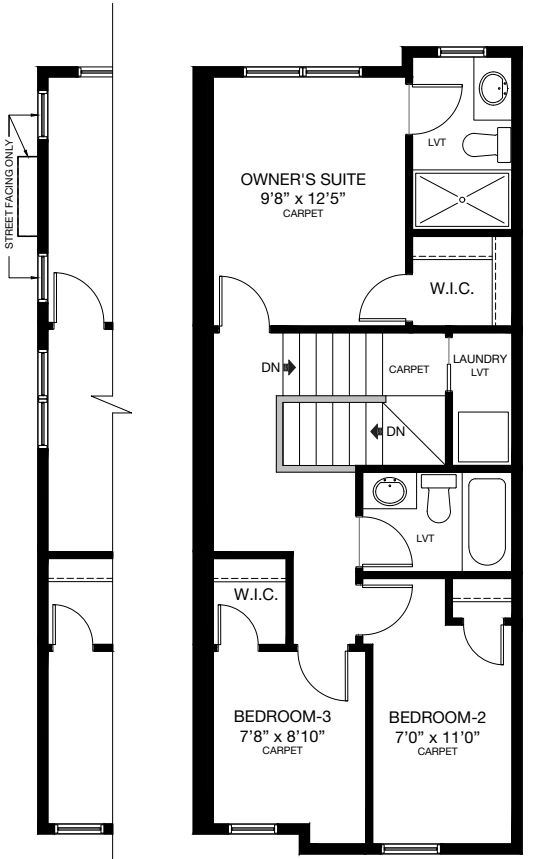
UPPER FLOOR MID UNIT Area: 579 Sq.Ft.
