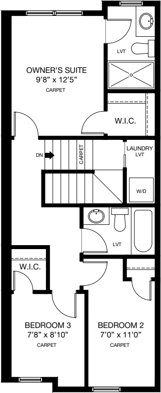
UPPER FLOOR MID UNIT Area: 579 Sq.Ft.
