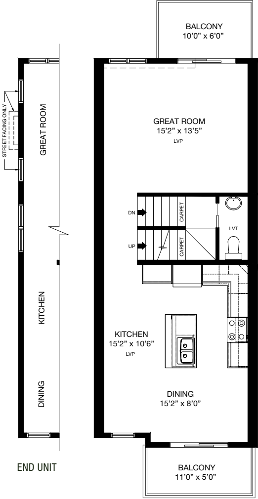
MAIN FLOOR Area: 643 Sq.Ft.
