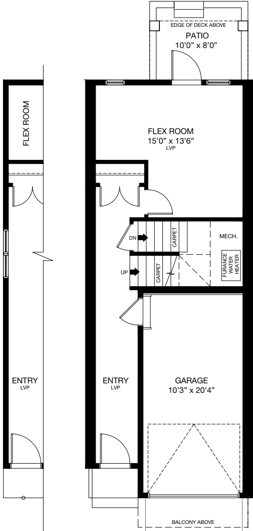
ENTRY LEVEL Area: 372 Sq.Ft.
