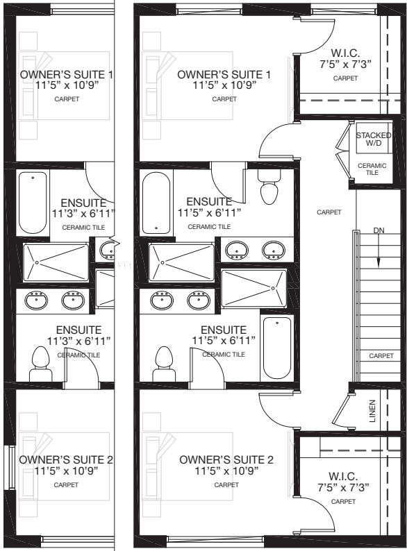
END UNIT UPPER LEVEL • OPTION 2 Area: 750 Sq.Ft. Total Area: 1834 Sq.Ft.
