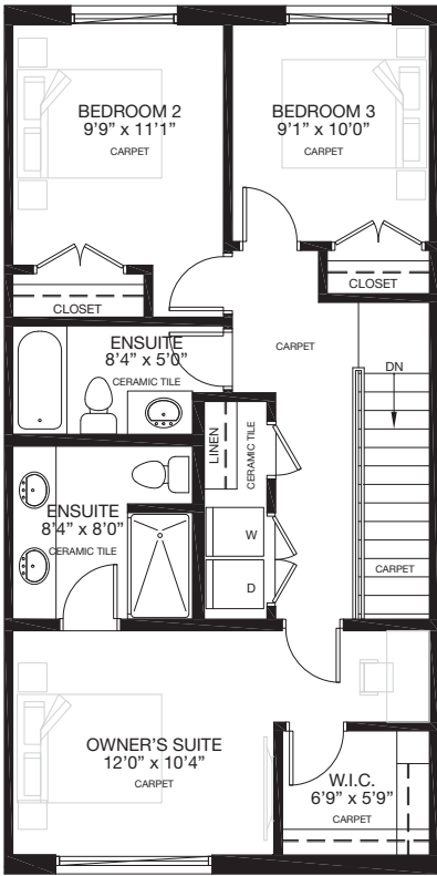
UPPER LEVEL Area: 750 Sq.Ft.
