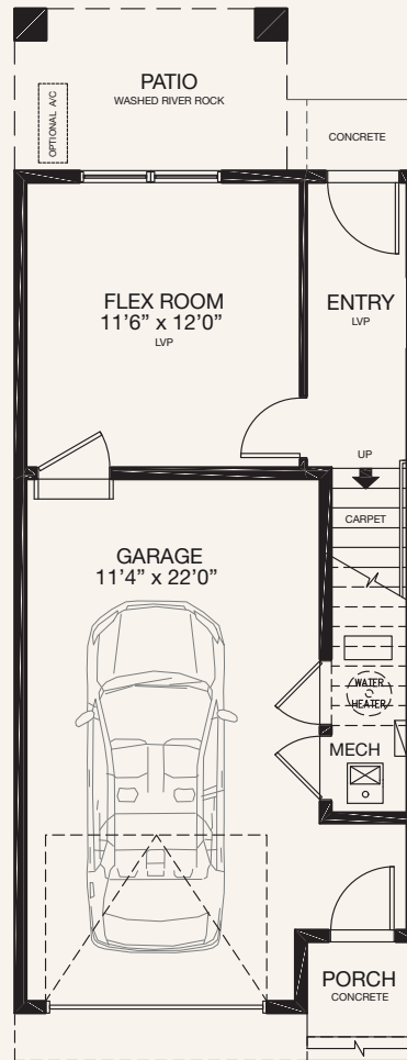
ENTRY LEVEL FLEX ROOM OPTION 1
