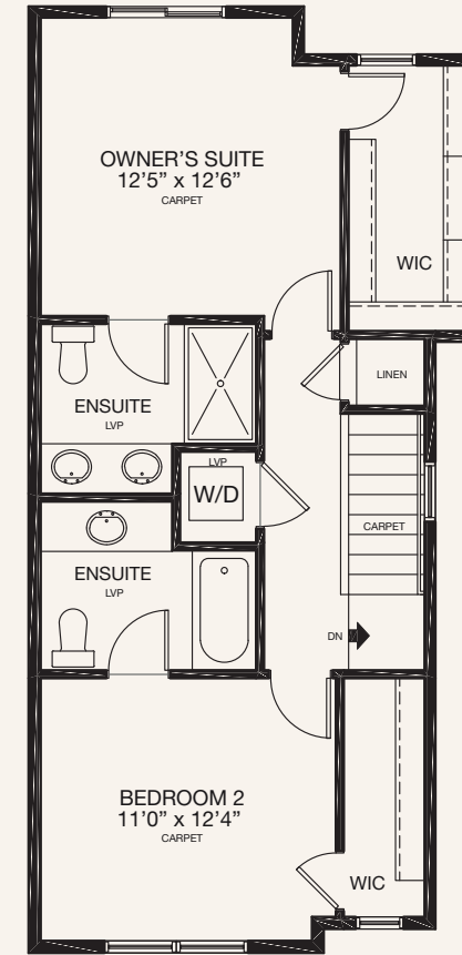
UPPER LEVEL DUAL BED OPTION
