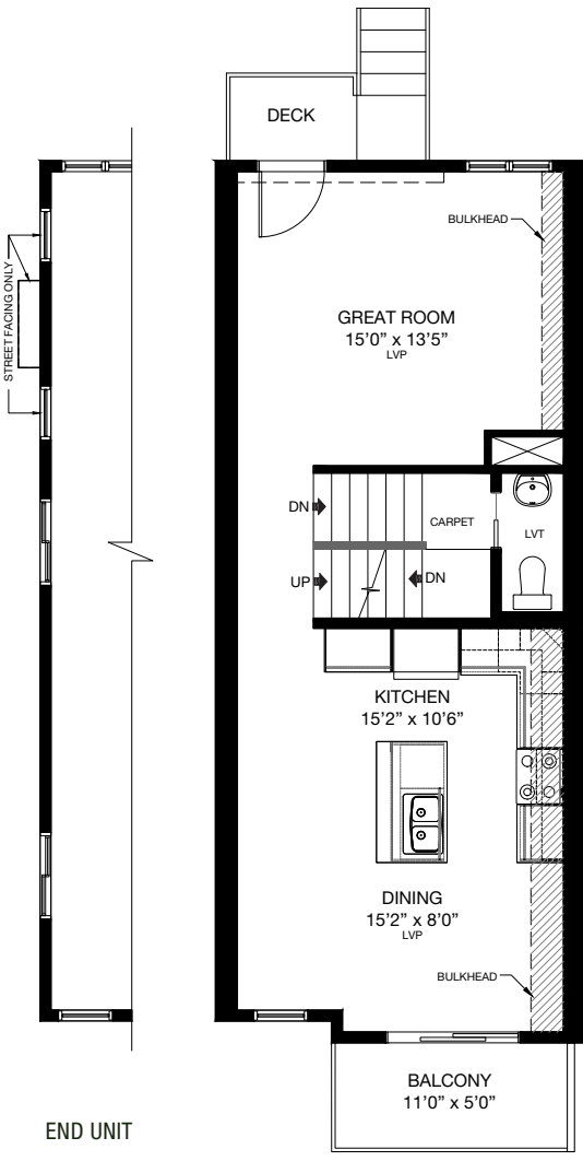
MAIN FLOOR Area: 643 Sq.Ft.
