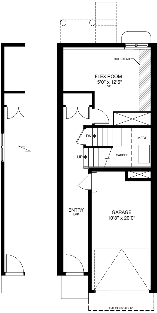
ENTRY LEVEL Area: 372 Sq.Ft.
