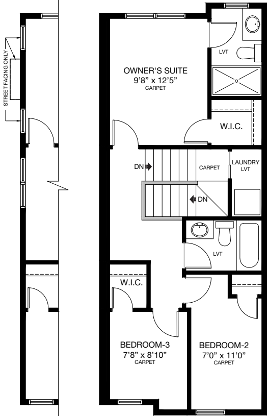
UPPER FLOOR MID UNIT Area: 579 Sq.Ft.
