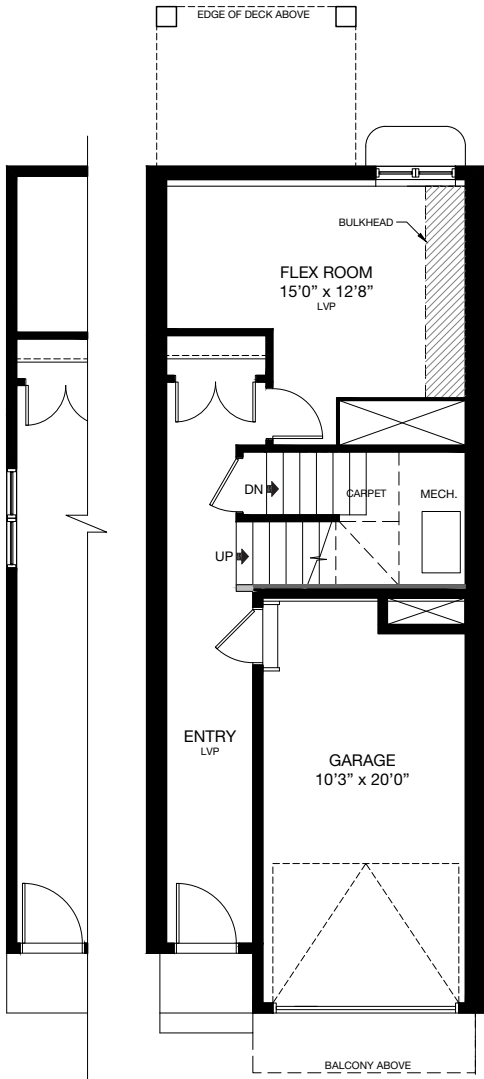
ENTRY LEVEL Area: 372 Sq.Ft.
