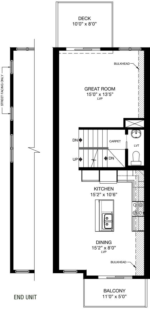
MAIN FLOOR Area: 643 Sq.Ft.
