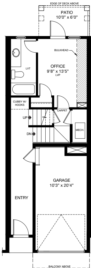
ENTRY LEVEL OPTION Area: 410 Sq.Ft.
