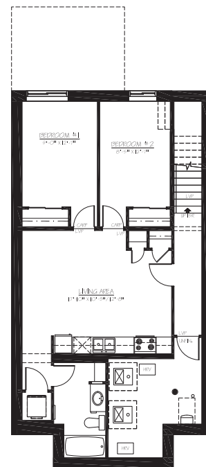
SECONDARY SUITE 759 SQ.FT
