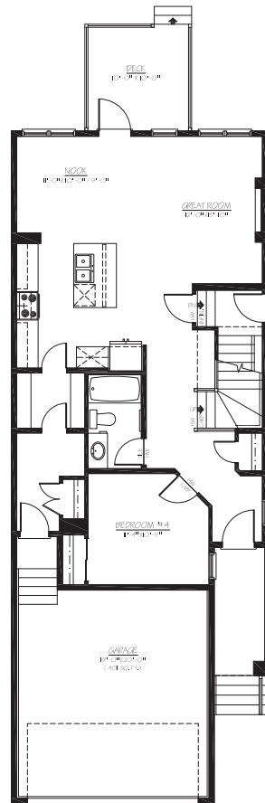
MAIN 991 SQ.FT
