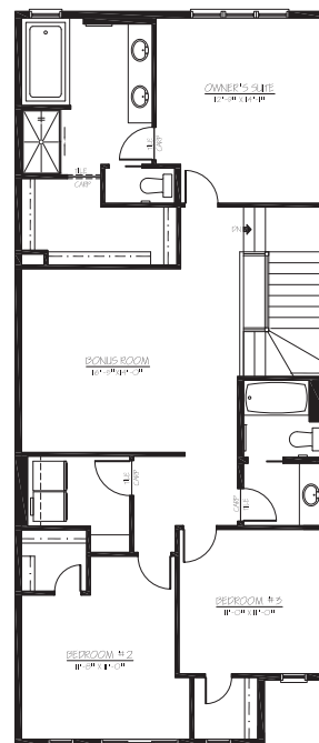
UPPER 1310 SQ.FT
