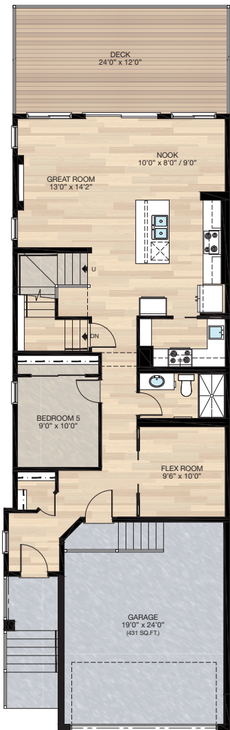
MAIN 1124 SQ.FT.
