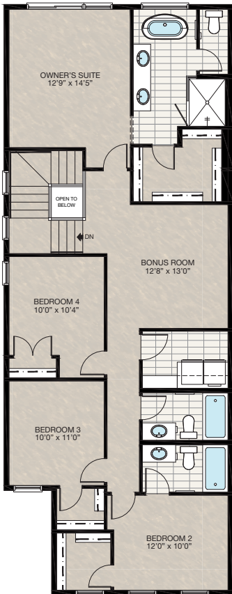
UPPER 1422 SQ.FT.
