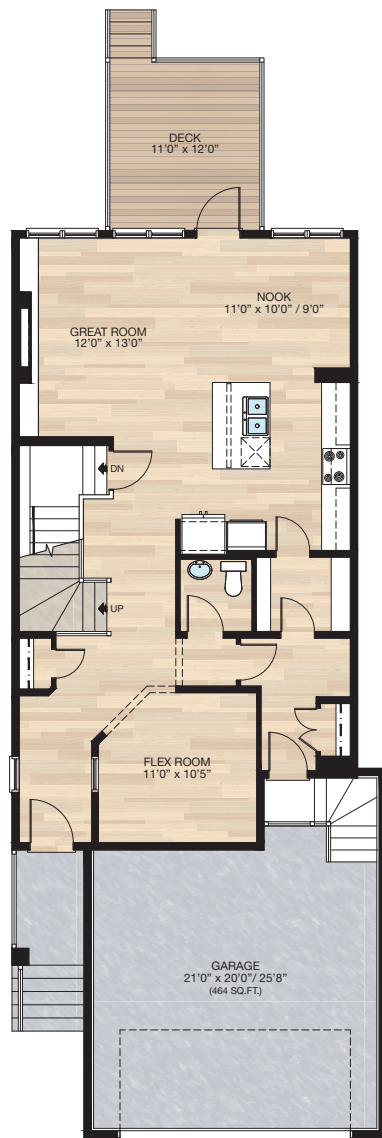
MAIN 1000 SQ.FT.
