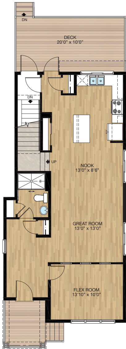
MAIN 915 SQ.FT.
